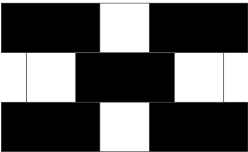
BUTTONS & BATTENS | LAYOUT 2 30x30 .12"x14" 66,67% 30x60 .12"x24" 33,33%
