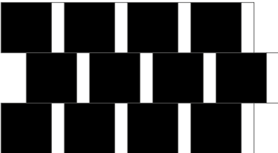
BUTTONS & BATTENS | LAYOUT 4 30x30 .12"x14" 80,65% 30x60 .12"x24" 19,35%
