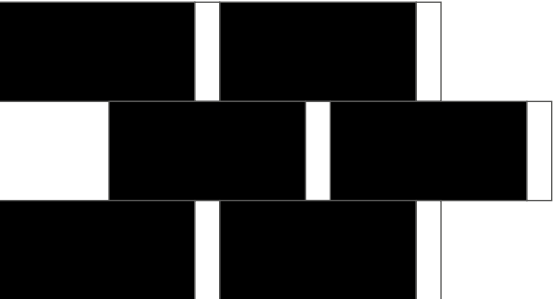
BUTTONS & BATTENS | LAYOUT 3 7,2x30 .3"x12" 89,29% 30x60 .12"x24" 10,71%
