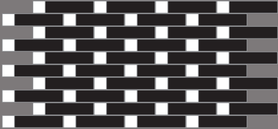
BUTTONS & BATTENS | LAYOUT 1 7,2x30 . 3"x12" 80,65% 7,2x7,2 . 3"x3" 19,35%
