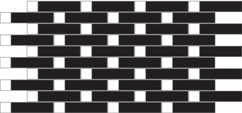
BUTTONS & BATTENS | LAYOUT 1 7,2x30 . 3"x12" 80,65% 7,2x7,2 . 3"x3" 19,35%
